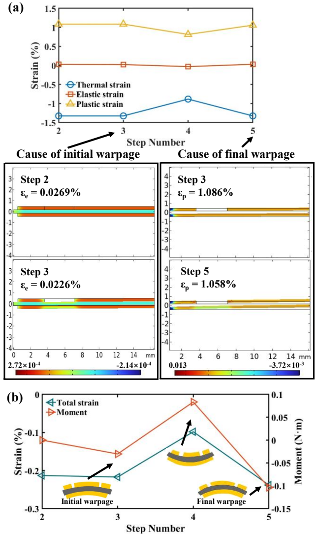
Figure 7. (a) Average strain in Cu layers from Step 2 to Step 5. The strain change that caused the initial and final warpage was displayed in the frames. (b) Evolution of moment and total strain from Step 2 to Step 5.
