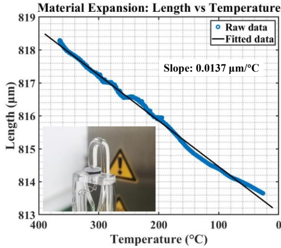
Figure 4. Evolution of annealed OFC expansion in the cooling phase from 365 °C to 25 °C. The inserted frame shows how the thickness is measured.
