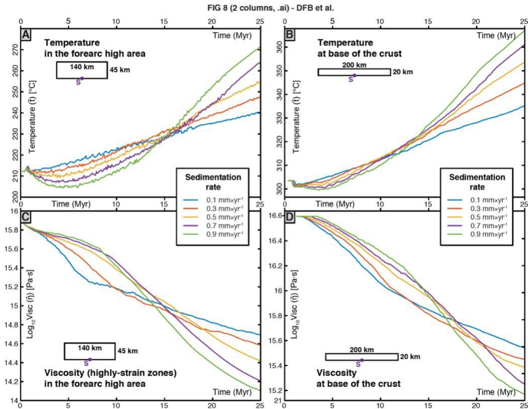
Figure 8. Temperature and viscosity variation of the forearc high and crustal base with sediment fill level.
