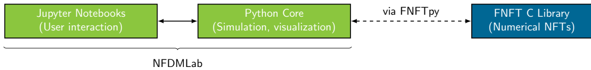
Fig. 2: Overview of components in NFDMLab.
