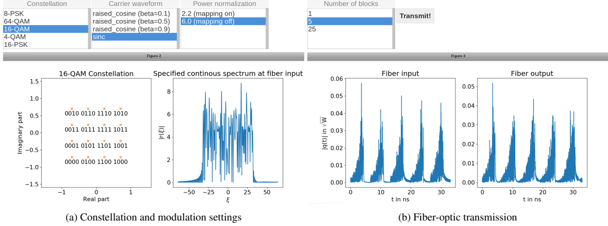
Fig. 1: Screenshots taken from a NFDMLab Jupyter notebook (work in progress).
