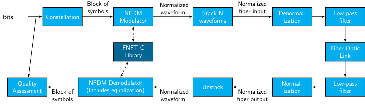
Fig. 3: Schematic representation of the Python core. The arrows indicate a typical workflow.
