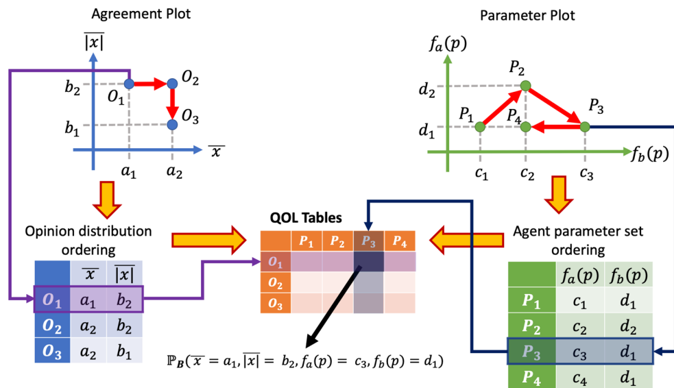
Figure 2. Construction of QOL Tables . Each of the points in the Agreement Plot has coordinates ((\bar{x})_i, (|\bar{x}|)_i) corresponding to a set O_i ; they are ordered as O_1, O_2, O_3 following the red arrows. Analogously, each of the points in the Parameter Plot has coordinates (p_{a,j}, p_{b,j}) corresponding to a set P_j ; they are ordered as P_1, P_2, P_3, P_4 following the red arrows. Then, the QOL Tables are constructed, whose rows are associated with points in the Agreement Plot and whose columns are associated with points in the Parameter Plot, in the corresponding order. Therefore, the cell in position (i, j) in the QOL Tables is associated with point O_i = ((\bar{x})_i, (|\bar{x}|)_i) in the Agreement Plot and with point P_j = (p_{a,j}, p_{b,j}) in the Parameter Plot, and contains a value between 0 and 1 that represents the probability \mathbb{P}_B .
