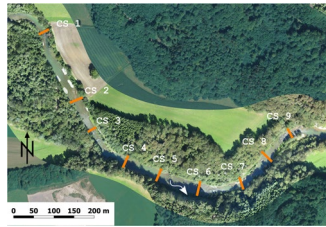
Figure 6. Nine cross-sections (CS) where flow depths and velocities were measured. CS 2–4 correspond to the HMID impact zone , CS 1 and 5–9 to the HMID rest zone (see Table 1). Background © Research unit Ecohydrology, ZHAW.
