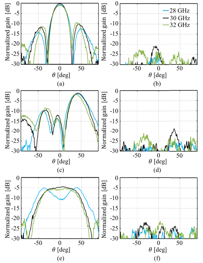
Fig. 15. Measured and normalized E-plane patterns of the array for several frequencies in broadside direction (a) co- and (b) cross pol., scanning to 45^\circ (c) co- and (d) cross pol., and the wide beam (e) co- and (f) cross pol. All patterns are normalized to the maximum of broadside array at 30 GHz.
