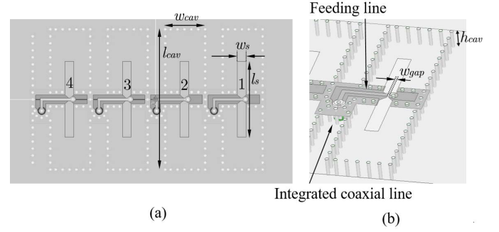
Fig. 9. (a) Top view of the slot array. (b) 3-D view of an array element with feeding structure.
