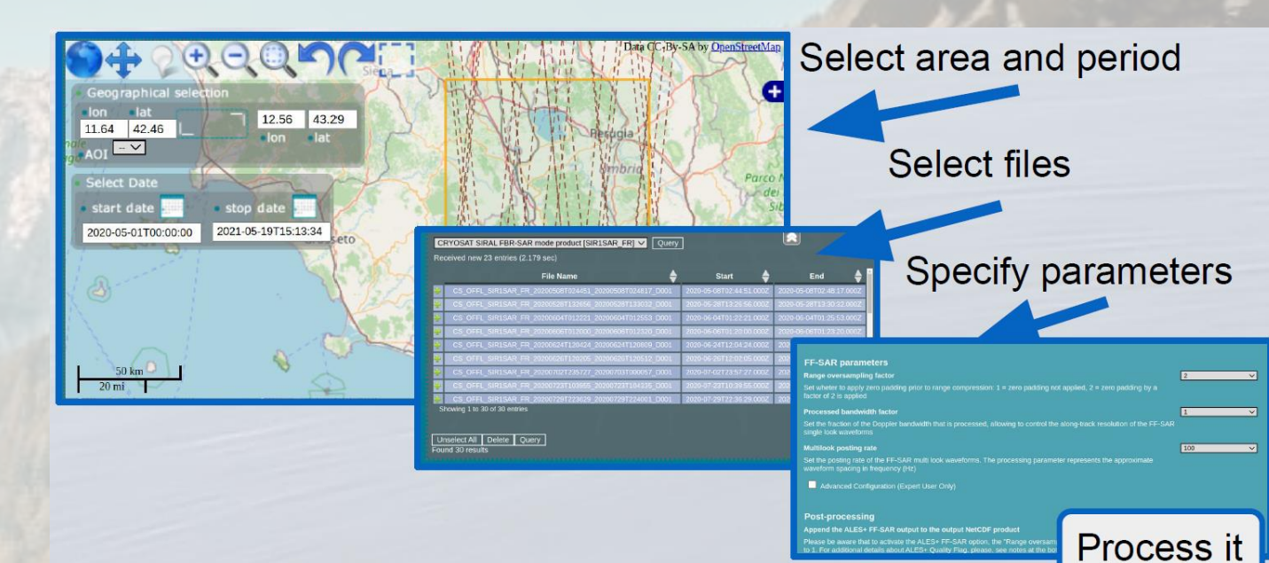
Figure 2: G-POD parameters and area of interest selection for FF-SAR processing.
