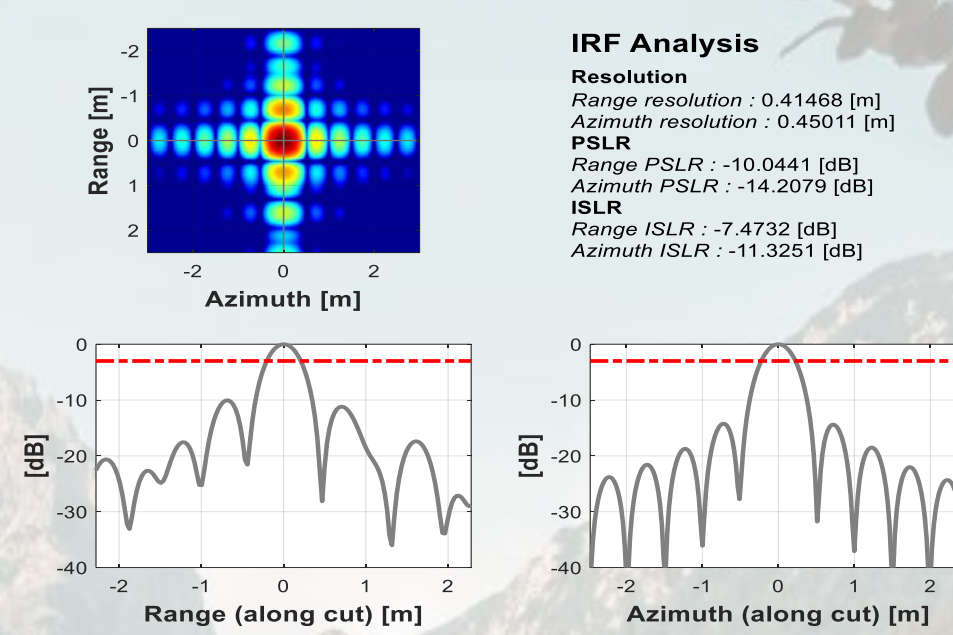
Figure 1: FF-SAR Point Target Response for CryoSat-2 acquisition over transponder obtained with AREALT-FF1 Processor Prototype.
