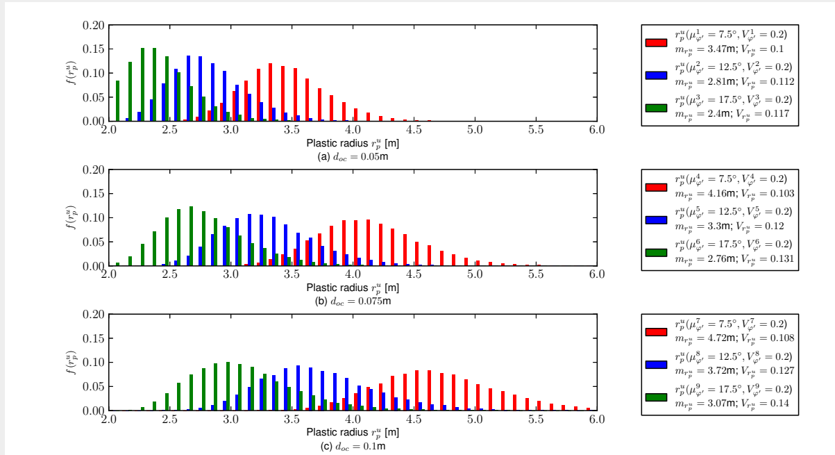
Figure 7.15.: Frequencies of plastic radii r_p for three mean friction angles \mu_{\phi'} and three different overcuts d_{oc} for a HLW gallery ( r_c = 1.6\text{m} ) at 500m depth.
