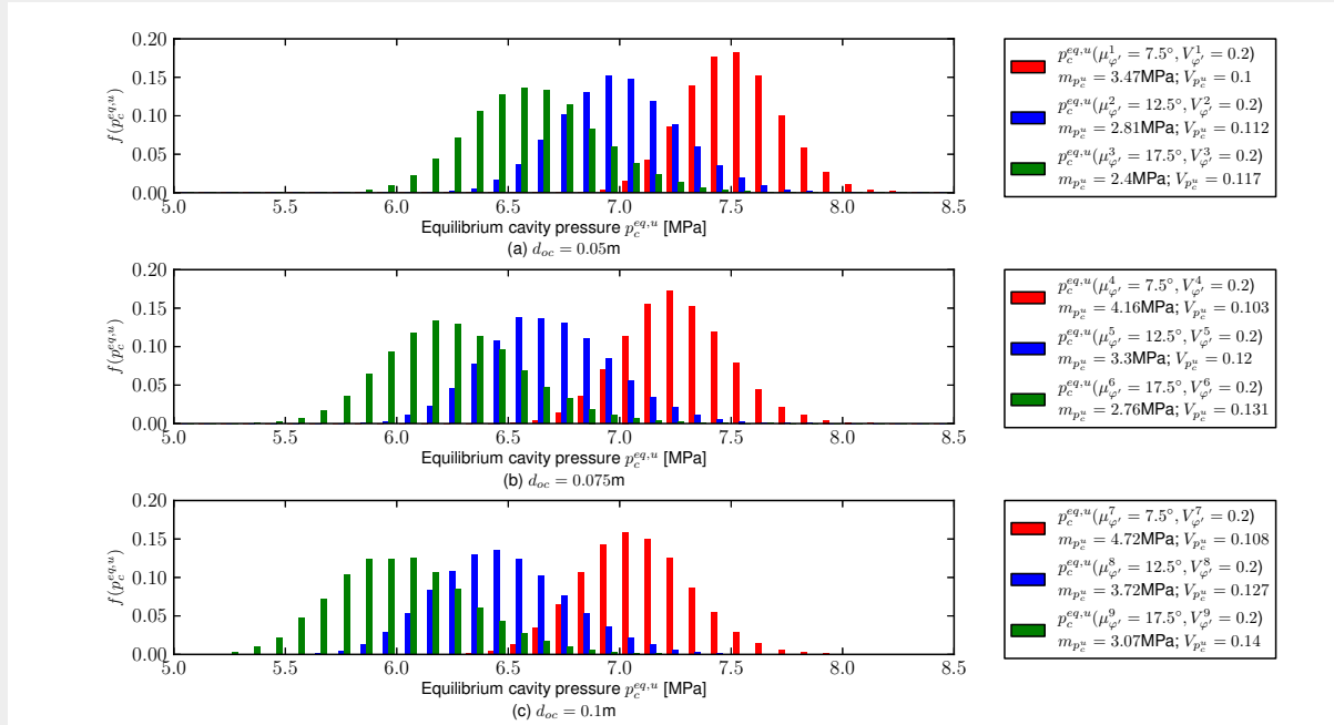
Figure 7.16.: Frequencies of equilibrium cavity pressure p_c^{eq} for three mean friction angles \mu_{\phi'} and three different overcuts d_{oc} for a HLW gallery ( r_c = 1.6\text{m} ) at 500m depth.
