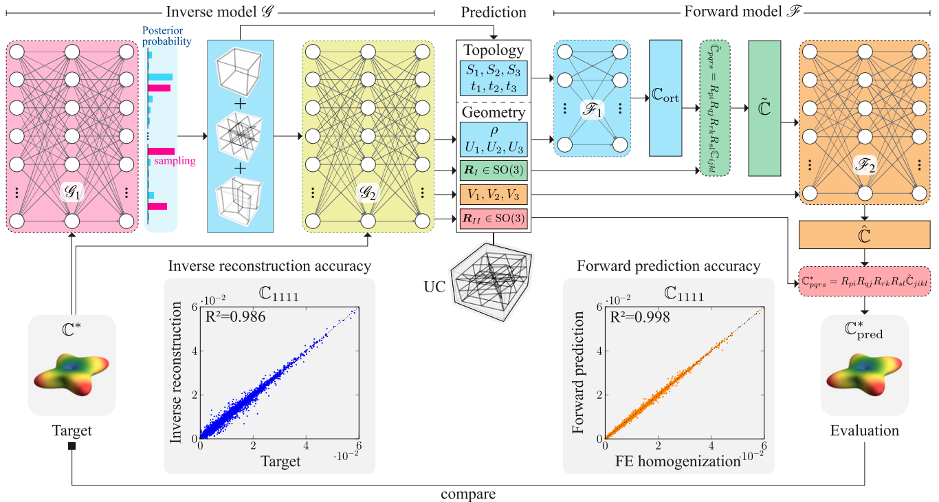
Fig. 2. Framework to generate truss lattices with given stiffnesses. The inverse model takes the 21 independent elastic constants of \mathbb{C}^* as input and first predicts a posterior distribution of possible lattice topologies, from which one (composite) topology is sampled and passed, jointly with \mathbb{C}^* , to a second NN, which predicts the corresponding geometrical parameters. The stiffness of the proposed lattice candidate is then reconstructed with the (independently trained) forward model and compared to the target stiffness. Predictions for \mathbb{C}_{1111} of the forward and inverse models are compared to the actual stiffness (obtained via FE modeling and the forward model, respectively) and the corresponding R^2 deviations indicated (evaluated on a test set of 30,000 truss lattices). Further details of the NN architecture, training schemes, and accuracy are summarized in SI Appendix, section 3.
