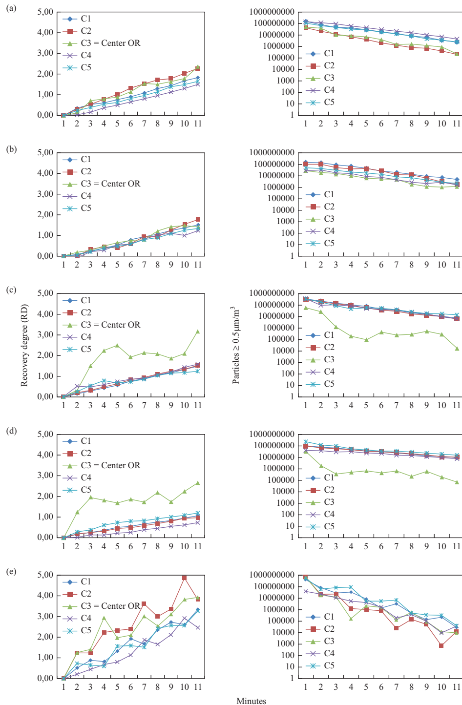
Figure 2. (a). The RD 10LV (left), recovery degree within 10 min low volume, and decay of airborne particles concentration CRR LV (right), cleanliness recovery rate per min low volume at row C1 -C5 of the CV LV , conventional ventilation system low volume. (b) The RD 10LV (left), recovery degree within 10 min low volume, and decay of airborne particles concentration CRR LV (right), cleanliness recovery rate per min low volume at row C1 -C5 of the cdV LV , controlled dilution ventilation system low volume. (c) The RD 10LV (left), recovery degree within 10 min low volume, and decay of airborne particles concentration CRR LV (right), cleanliness recovery rate per min low volume at row C1 -C5 of the TcAF LV , temperature-controlled airflow system low volume. (d) The RD 10LV (left), recovery degree within 10 min low volume, and decay of airborne particles concentration CRR LV (right), cleanliness recovery rate per min low volume at row C1 -C5 of the UDAF LV-1 , uni directional airflow-1 system low volume. (e) The RD 10LV (left), recovery degree within 10 min low volume, and decay of airborne particles concentration CRR LV (right), cleanliness recovery rate per min low volume at row C1 -C5 of the UDAF LV-2 , uni directional airflow-1 system low volume.
