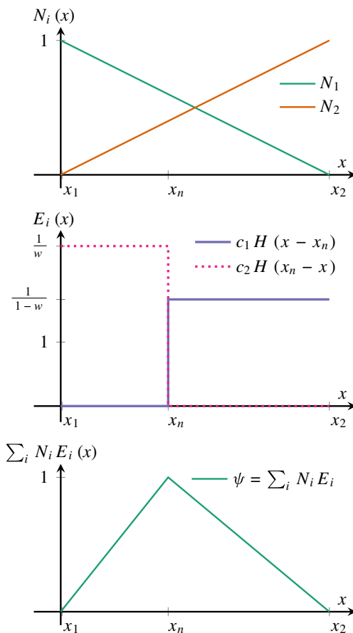
Fig. 22 Construction of IGFE enrichment function from X/GFEM formulation
