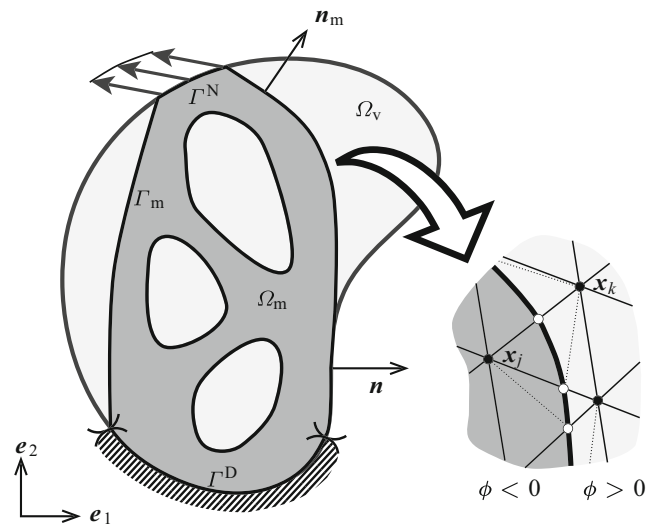
Fig. 1 Mathematical representation of a topology optimization design domain \Omega . Essential and natural boundary conditions are prescribed on the part of the boundary denoted \Gamma^D and \Gamma^N , respectively. The material domain is referred to as \Omega_m , while the void region is denoted \Omega_v . The inset shows the discretization with a material interface, defined by the zero-contour of the level set function \phi , that is non-matching to the mesh. Original mesh nodes and enriched nodes are denoted with black circles \bullet and \circ white circles, respectively
