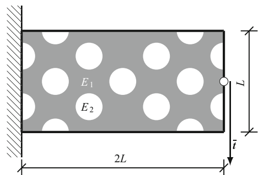
Fig. 7 Problem description and initial design for the cantilever beam example in Section 3.2. The domain is clamped on the left and a downward force is applied in the middle of the right side
