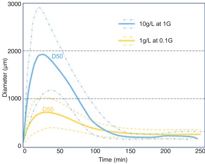
Fig. 7.18 Sediment plume aggregation dynamics in the water column simulator. d_{50} (solid lines \pm STD (dashed lines) from particle camera data, analysed with Matlab
