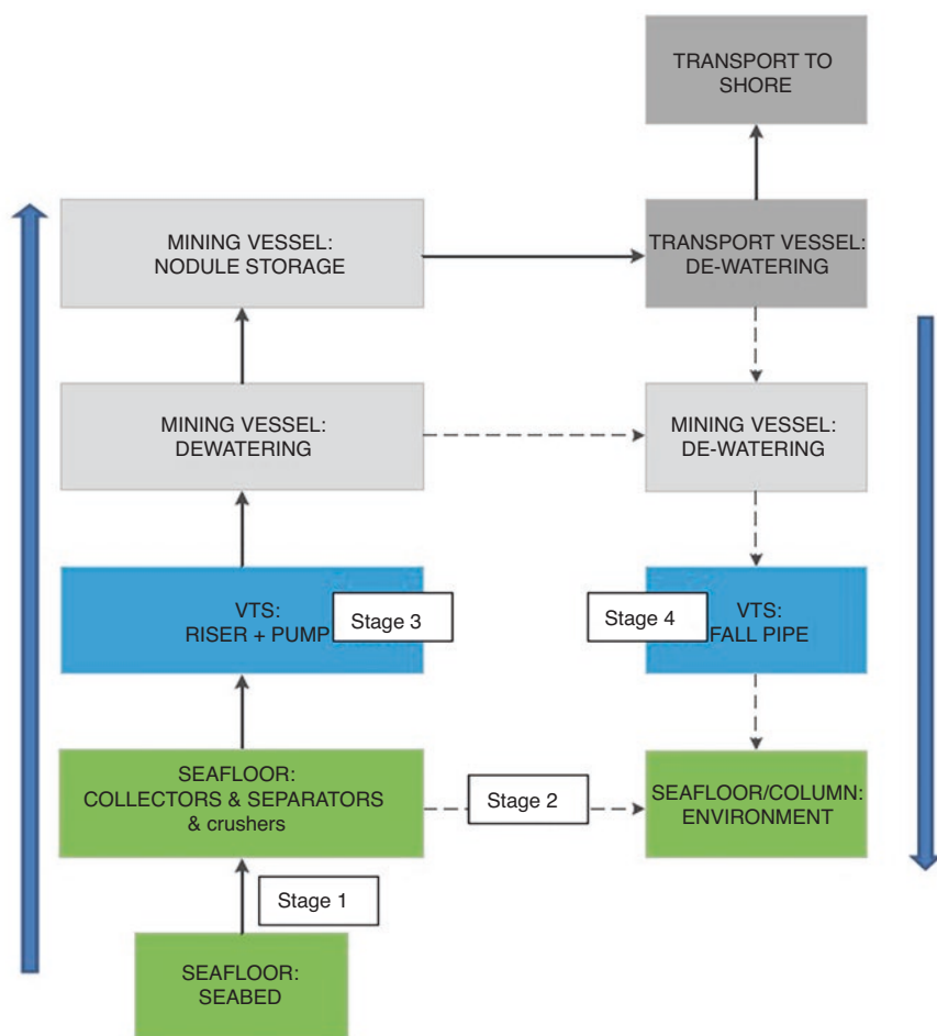
Fig. 7.1 Schematic of material flows. Solid lines represent the main flow (noodles) and dashed lines represent secondary flow (sediments, waste, and other effluants, SWOE). Blue arrows show the general direction of the flow. (Based on Blue Nodules Lang et al., 2019)
