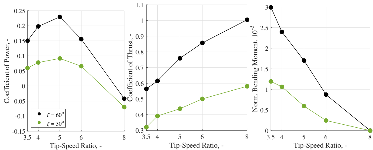
Fig. 21 Static response results, variable tower tilt angle at \Omega = 600RPM , \beta = 0^\circ with stiff blades rotor
