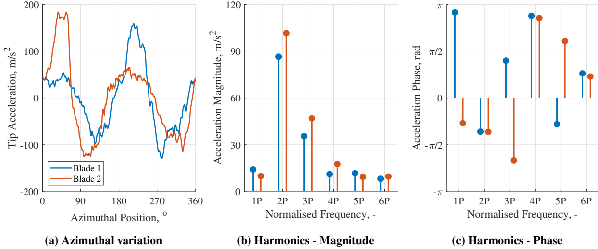
Fig. 14 Kinematic symmetry between the two flexible blades at \xi = 30^\circ , \Omega = 600RPM , \beta = 0^\circ and \lambda = 3
