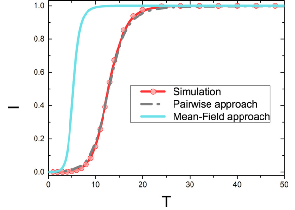
Fig. 3. Comparison of simulation results with the mean-field model and the pair approximation model without considering the effect of adaptive process. The horizontal axis ( T ) is the time step for the Monte Carlo simulation, the vertical axis ( I ) is the density of infected. The parameters are set as \beta = 0.3 , \sigma_S = 0.5 , \sigma_I = 0.7 , \lambda = 0.2 , \omega = 0.75 , \alpha = 0.6 , r_S = r_I = 0 .
