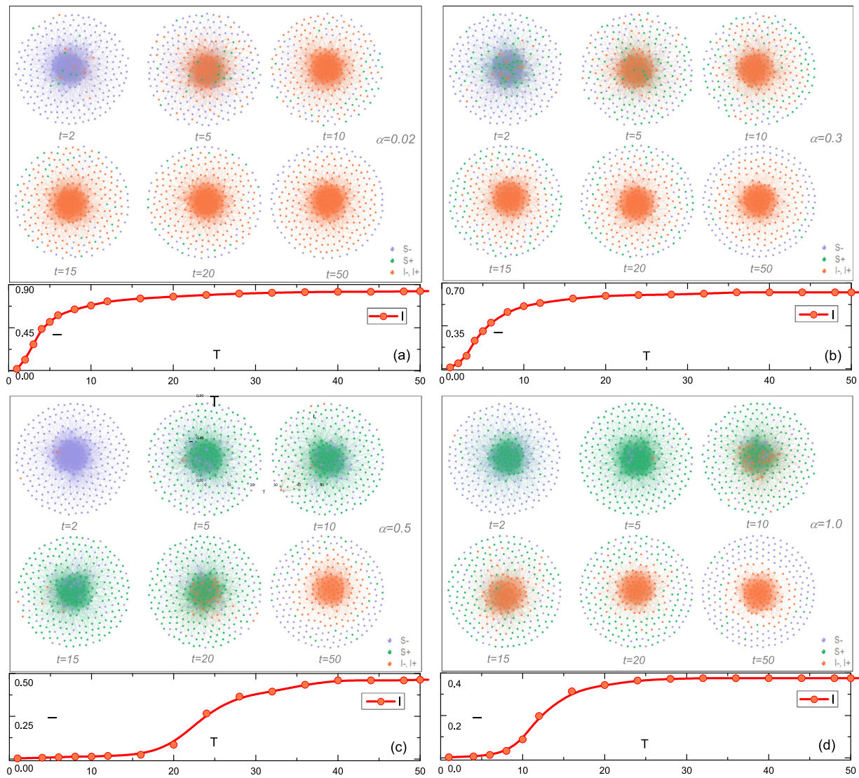
Fig. 7. Illustration to dynamic spreading process by considering the adaptive effect on haggie network, while the purple, green and red circles represent individuals in S^- , S^+ and I state respectively. The red curves (lower panels) describe the fraction of infected individuals over time with corresponding parameters. (a) \alpha = 0.02 ; (b) \alpha = 0.3 ; (c) \alpha = 0.5 ; (d) \alpha = 1.0 . Other parameters are set as \beta = 0.1 , \sigma_S = 0.3 , \sigma_I = 0.5 , \lambda = 0.08 , \omega = 0.2 , r_S = r_I = r = 0.08 . (For interpretation of the references to color in this figure legend, the reader is referred to the web version of this article.)
