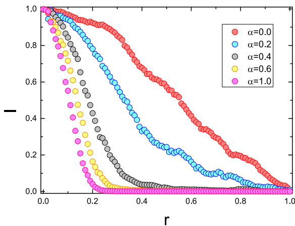
Fig. 8. Final fraction of infected individuals versus r . Different curves correspond to different \alpha . Other parameters are set as \beta = 0.2 , \sigma_s = 0.5 , \sigma_I = 0.7 , \lambda = 0.2 , \omega = 0.2 .
