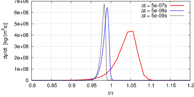
Figure 9: Evolution of dp/dt at r/R_0 = 0.25 for C_c = 250 \text{kg/s/m}^5 and different time step sizes
