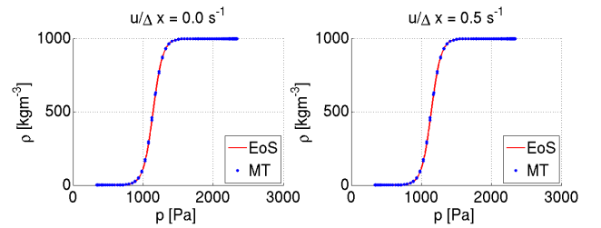
Figure 5: Density-pressure trajectories (MT) corresponding to Figures 3 and 4 and barotropic equation of state (EoS)
