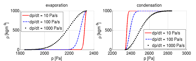
Figure 1: Density-pressure trajectories for different pressure change rates (compare to Schenke & Van Terwisga 2016)
