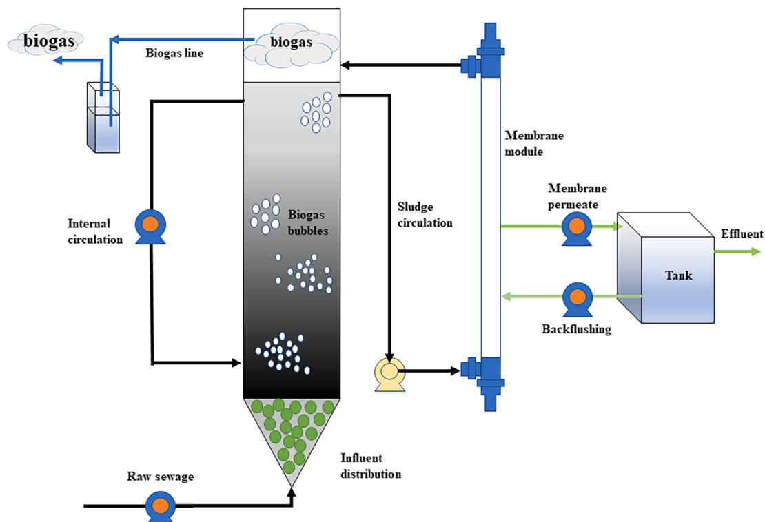
Fig. 1. Schematic view of an anaerobic membrane bioreactor.
