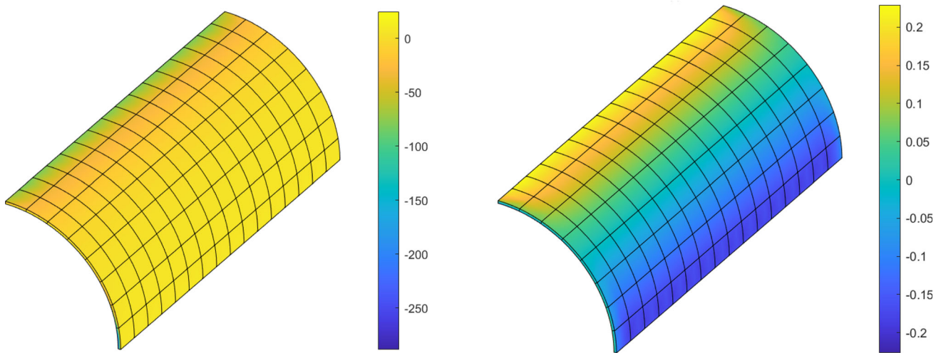
Fig. 17 Pinching of a cylinder. Contravariant stress components S^{11} (left) and covariant strains E_{33} + \zeta \bar{E}_{33} (right) for the inward case at \lambda = 0.667
