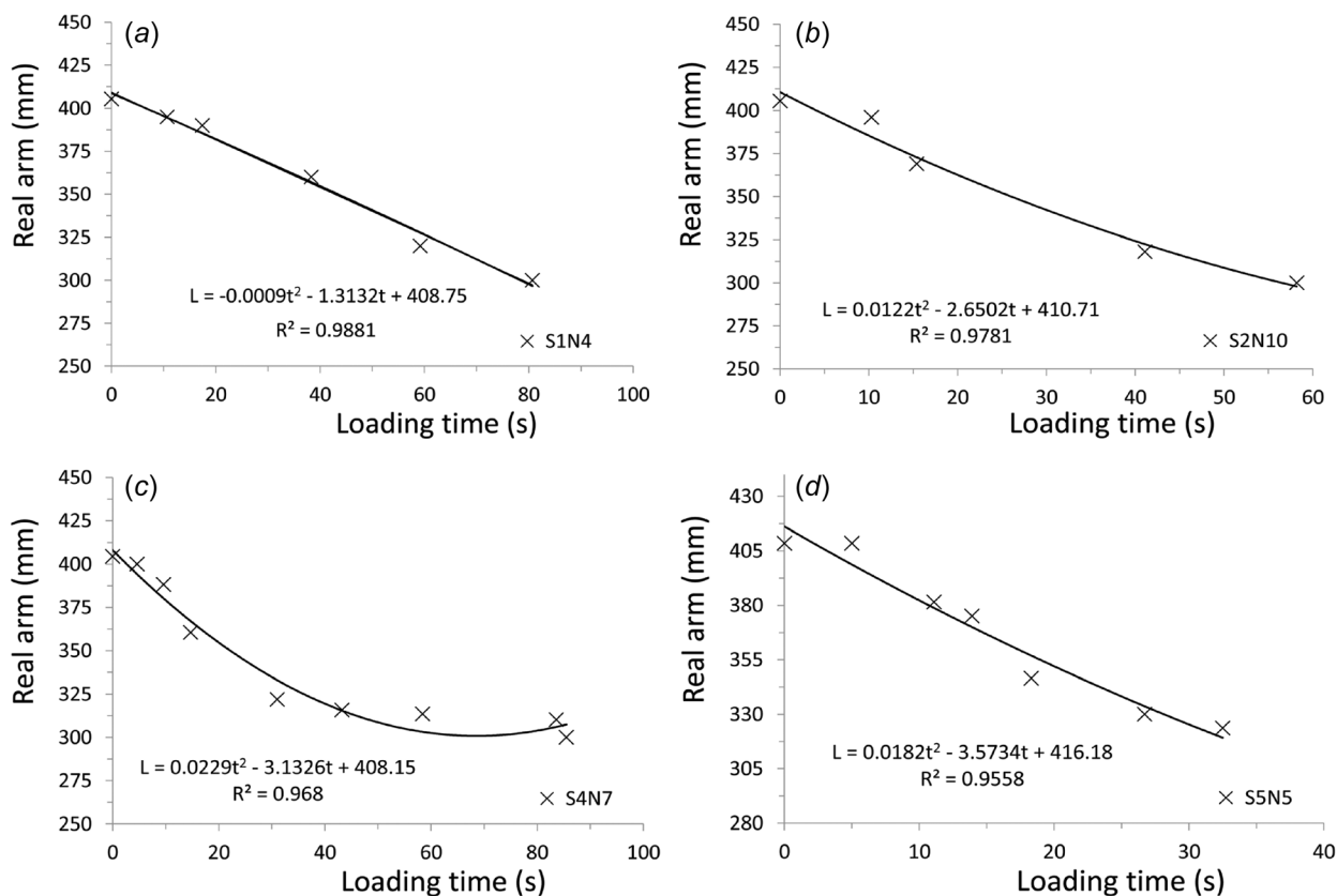
Fig. 13 The variation relationship between bending arm and loading time: (a) specimen S1N4, (b) specimen S2N10, (c) specimen S4N7, and (d) specimen S5N5
