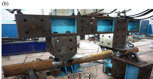
Fig. 3 The configuration of four-point bending structural test: (a) the design of bending test setup and (b) the real test setup in the laboratory
