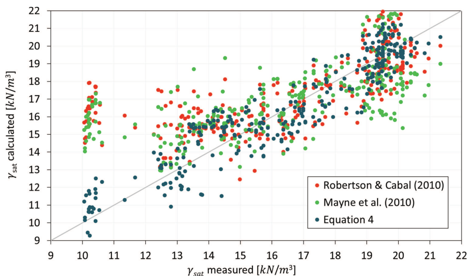
Figure 5. Measured versus calculated saturated unit weights using some of the different correlations from Table 4. Note that herein no cut-off value is applied for the minimum value of the calculated unit weight.
