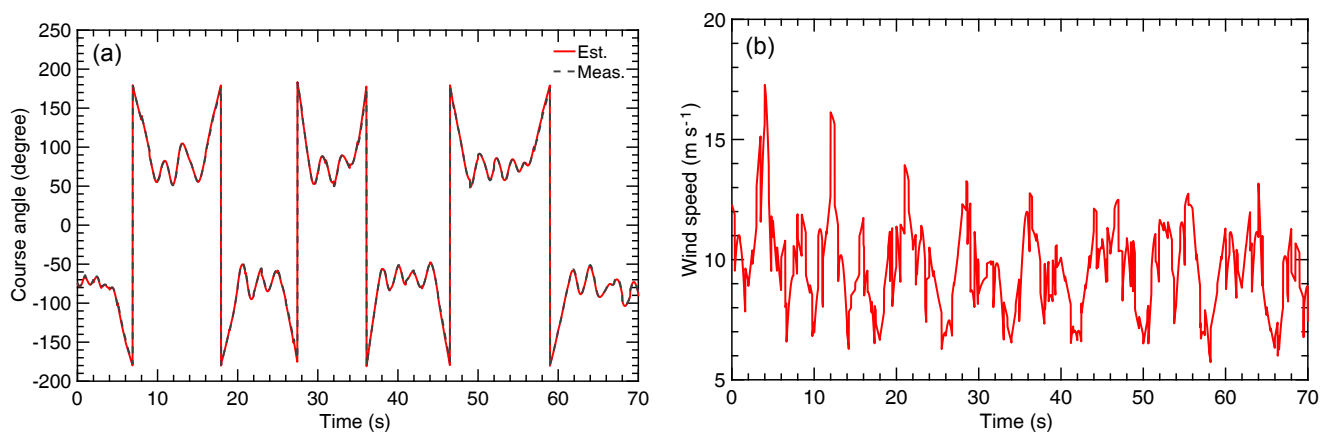
Figure 11. (a) Time history of the measured and estimated course angles. (b) Time history for the wind speed during the first flight condition.
