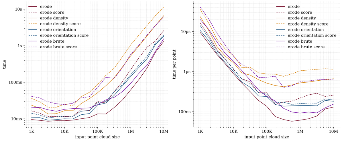
Figure 4.2 – Total runtime and time per SE point for the erosion variants, total time on the left, time per point on the right
