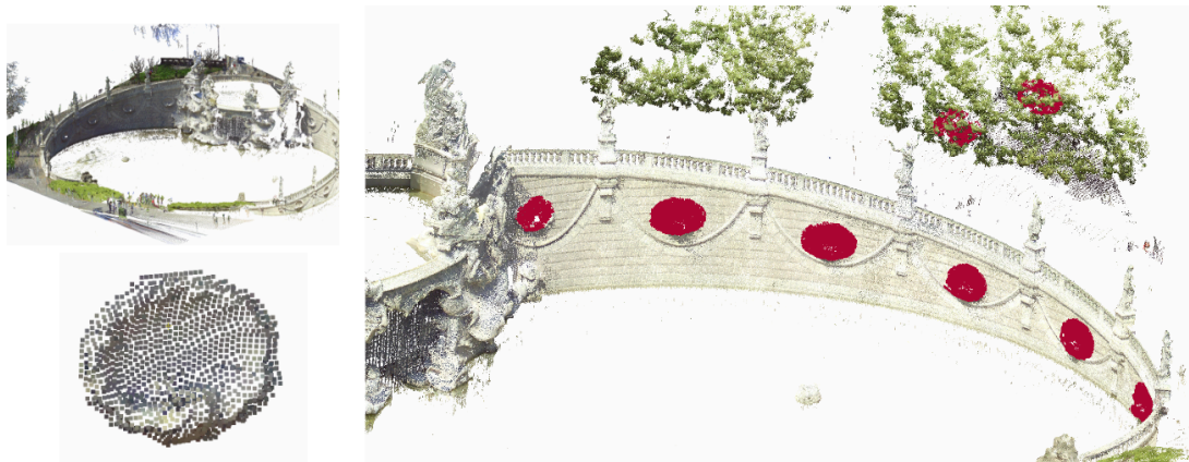
Figure 4.25 – Shell detection (red) in the FM dataset using the brute-force orientation opening
