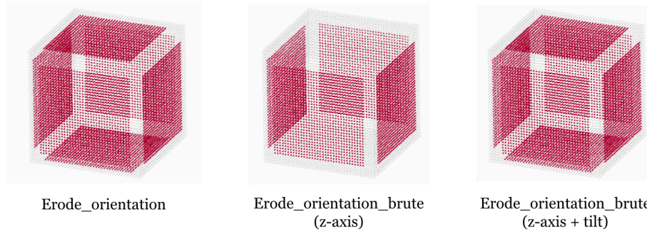
Figure 4.14 – Orientation-aware erosion on a hollow cube: full orientation erosion (left), brute-force restricted to z-axis rotations (centre), brute-force with z-axis and tilt (right)
