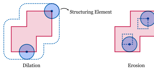
Figure 1.1 – Dilation and erosion applied to 2D shapes. Input shape in red, structuring element in blue, result of the operation indicated by the blue dashed line.
