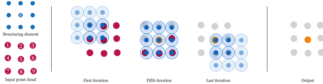
Figure 2.4 – Point-based erosion, input point cloud in red, structuring element in blue, resulting point cloud in yellow; source: (Balado et al., 2020)
