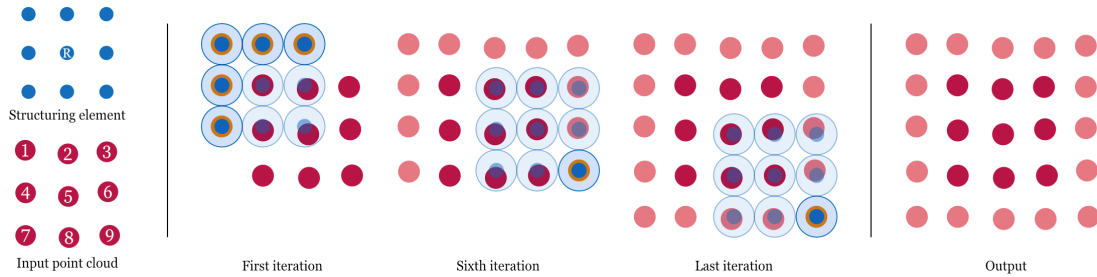
Figure 2.5 – Point-based dilation, input point cloud in red, structuring element in blue, resulting point cloud in red and pale red; source: (Balado et al., 2020)
