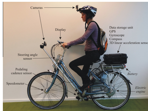
Fig. 1. The instrumentation of the pedelec. The instrumented conventional bicycle was not fitted with the battery and electric engine (indicated in italics ).
