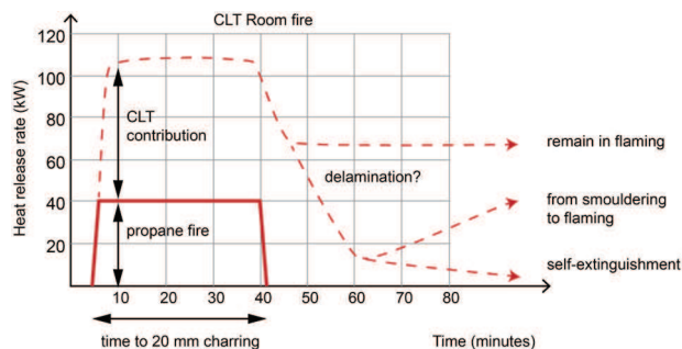
Figure 5: Approach of the second series of experiments
