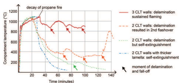
Figure 11: Compartment temperatures at 400 mm height in four of the samples of the second series of experiments
