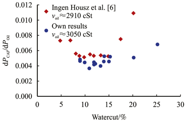
Fig. 4. Comparison of the current measurements for scaled pressure drop with those of Ingen Housz et al. [6].
