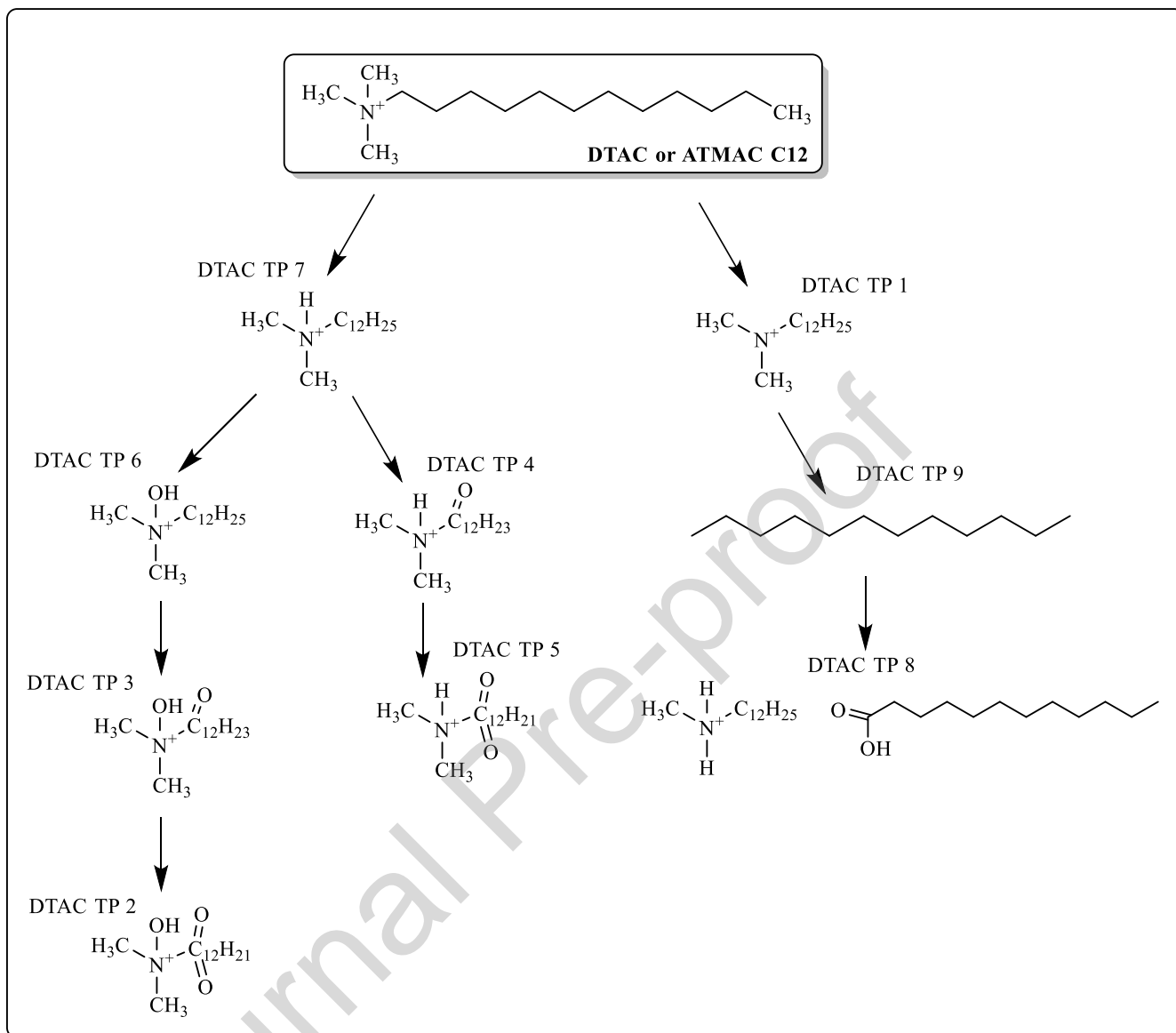
Figure 5: Proposed degradation pathway for DTAC in UV/PS/Cu 2+ (Reproduced with permission from (Lee et al., 2020))
