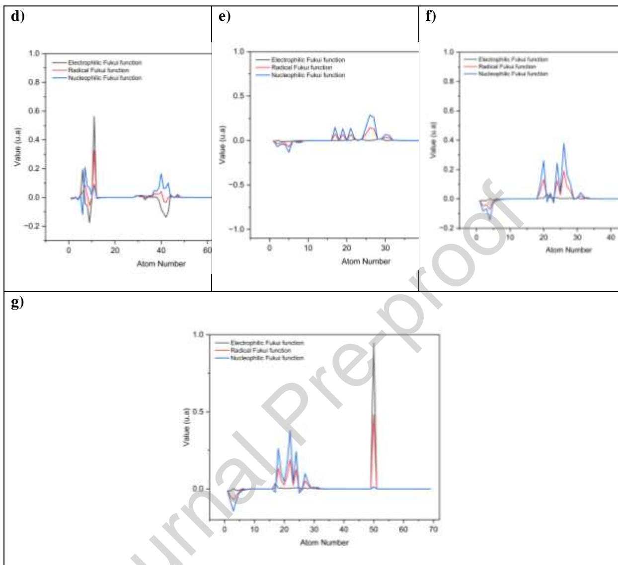
Figure 3. Representation of electrophilic, nucleophilic and radical Fukui functions of a) BAC C12, b) BAC C14, c) BAC C16, d) BAC C18, e) ATMAC C12, f) ATMAC C14 and g) ATMAC C18 at UM06-2X/6-311(2df,2pd) level of theory (Table S14-S18). Electrophilic, radical, and nucleophilic Fuki functions are represented by black, red, and blue lines, respectively.
