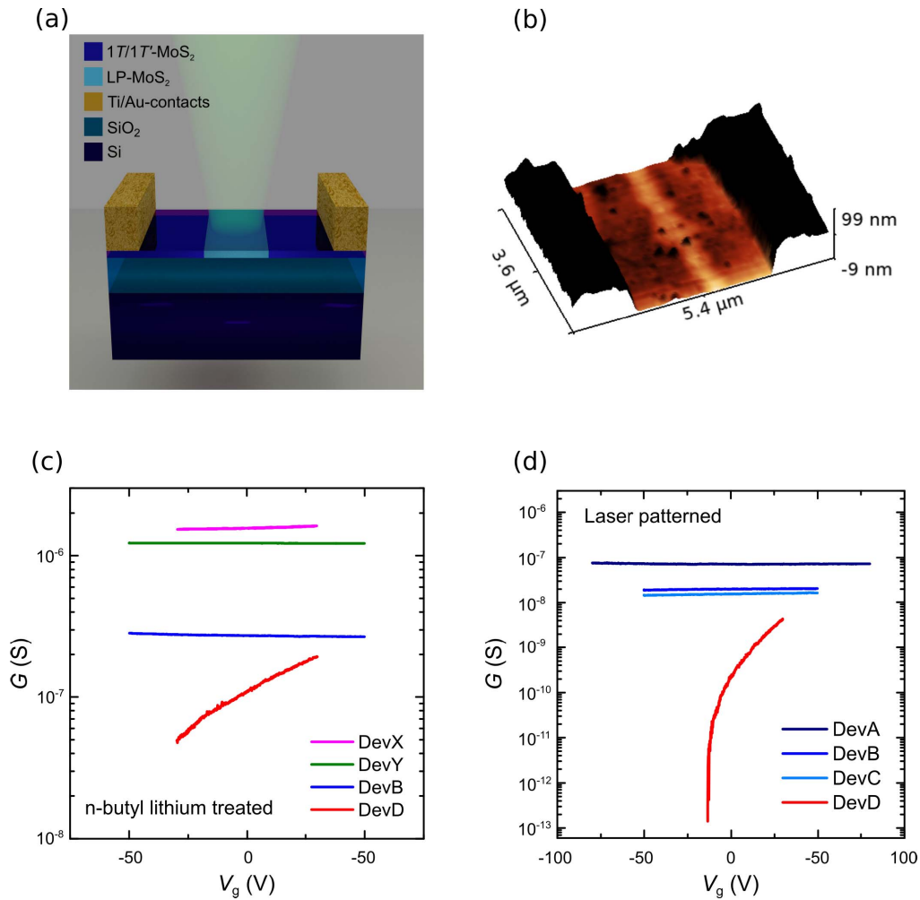
Fig. 3. Investigating the laser-induced phase transitions of a few-layer \text{MoS}_2 FET. (a) Illustration of a device, where the laser is patterning a strip of the flake to create the semiconducting 2H- \text{MoS}_2 channel. (b) 3-D AFM topographic image of a device (B) after LP of a narrow strip in the middle of the channel with a laser power of \sim 1 mW and spot size of 500 nm. The strip in the middle of the channel has an approximate width of 400 nm and corresponds well with the laser treated portion of the \text{MoS}_2 . (c) Conductance as a function of the back-gate voltage from four 1T/1T'- \text{MoS}_2 devices directly after the chemical treatment with BuLi. The poor modulation of the conductance from the back-gate voltage indicates the high-carrier-concentration in the devices. (d) Conductance as a function of the back-gate voltage from four devices after patterning a strip in the middle of the transistors as illustrated in (a) and shown in (b). In most devices, the modulation of the conductance from the back-gate voltage is still negligible, which illustrates the ineffective laser-induced phase change.
