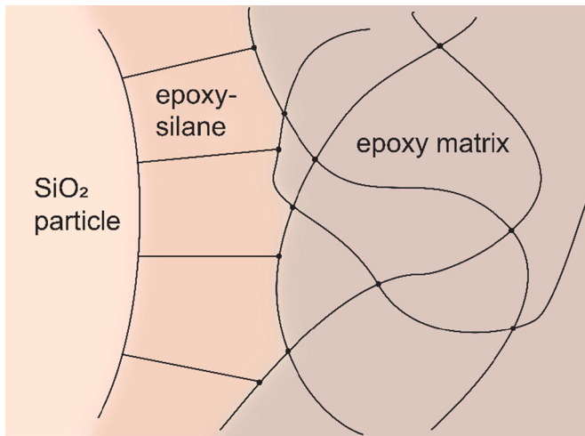
Fig. 1. Simplified schematic of interphase structure (not to scale). Epoxy silane molecules bind to the \text{SiO}_2 on one end and the epoxy matrix on the other end.
