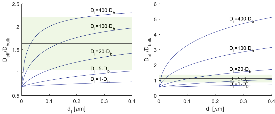
Fig. 11. Effective medium theory predictions for the effective diffusivity normalized by the bulk diffusivity ( D_{\text{eff}}/D_{\text{bulk}} ) at different interphase thicknesses ( d_i ), for a particle size of 2.9 \mu\text{m} , at filler volumes of 0.2 (left) and 0.3 (right); the solid lines mark the measured values at 30 °C. The green shadow gives the error of the measured value with 95% confidence bounds. The blue lines give the results of the EMT for various ratios of interphase diffusion compared to the bulk diffusion. (For interpretation of the references to colour in this figure legend, the reader is referred to the web version of this article.)
