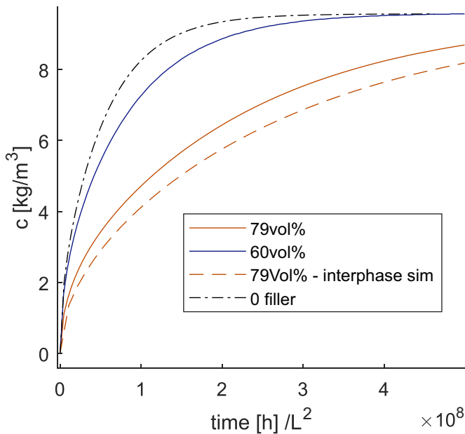
Fig. 13. Uptake simulation of EMC samples with different amount of fillers (water uptake (kg/m³) on epoxy volume considered for better comparison of uptake dynamics), dashed line: interphase simulation.
