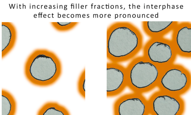
Fig. 14. Simplified schematic showing changes in volume fraction of the interphase with increasing particle density.
