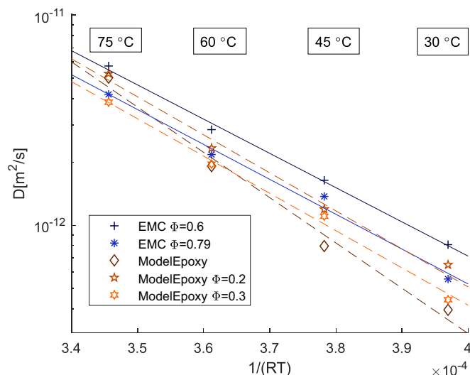
Fig. 10. Arrhenius plot of effective diffusivity as measured in DVS for a step in RH from 0 to 60%. The markers represent the measured values, while the lines show the Arrhenius fit; \phi is the filler level of the sample; error bars are lacking for better visibility, errors are 10%–20%, with exception of the model epoxy at \phi = 0.3 , which has errors of about 30% for 30 °C and 45 °C.
