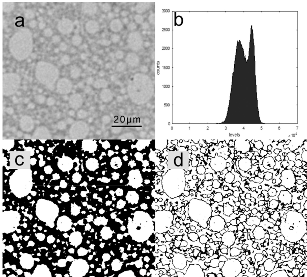
Fig. 4. Micro-CT image (1 slice) of EMC sample (79 vol%). (a) Image as obtained from the micro-CT scan, \text{SiO}_2 particles appear brighter than epoxy matrix. (b) Histogram of this image. (c) Pixels of lower peak in histogram (levels of 2 \times 10^4 to 4 \times 10^4 ) are ascribed a black value. (d) Pixels from max of epoxy peak to the minimum between the peaks are ascribed a black value.
