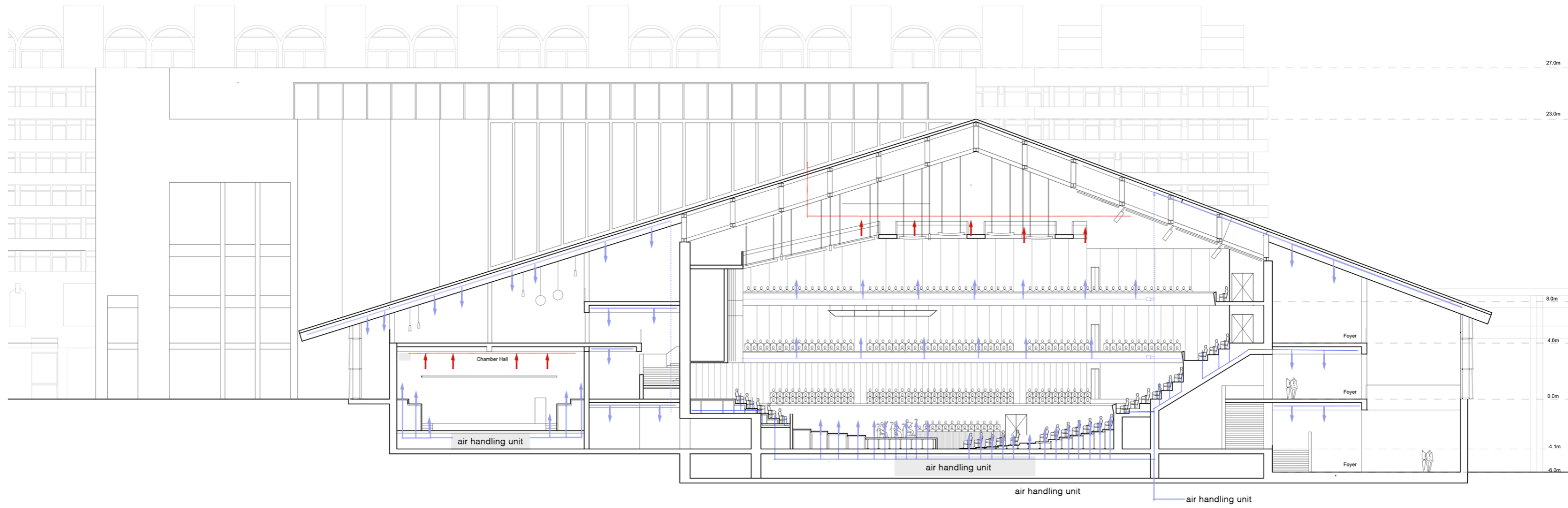
House of Music A-A Section 1:200
