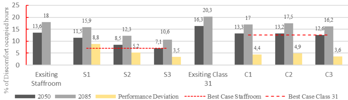
Figure 7 Robustness evaluation of selected strategies for staffroom and class 31 of Melanchthon School.
