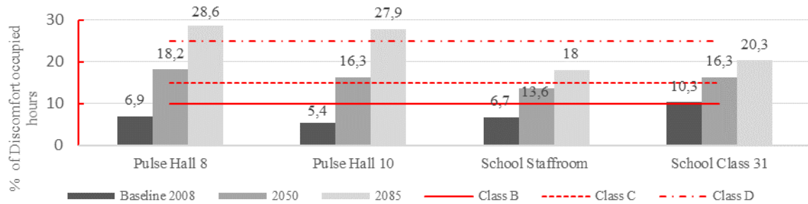
Figure 4 Comparison of percentage of discomfort hours due to overheating in baseline 2008, 2050 and 2085 climate scenarios.
