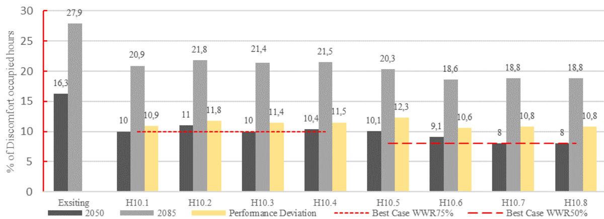
Figure 6 Robustness Evaluation of selected strategies for Hall 10 Pulse Building
