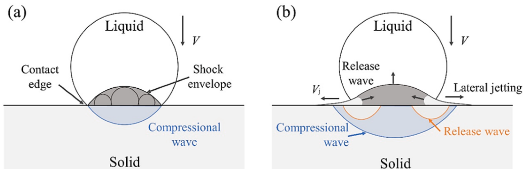
Fig 1. Liquid-solid impingement. (a) Liquid compression. (b) Lateral jetting.
