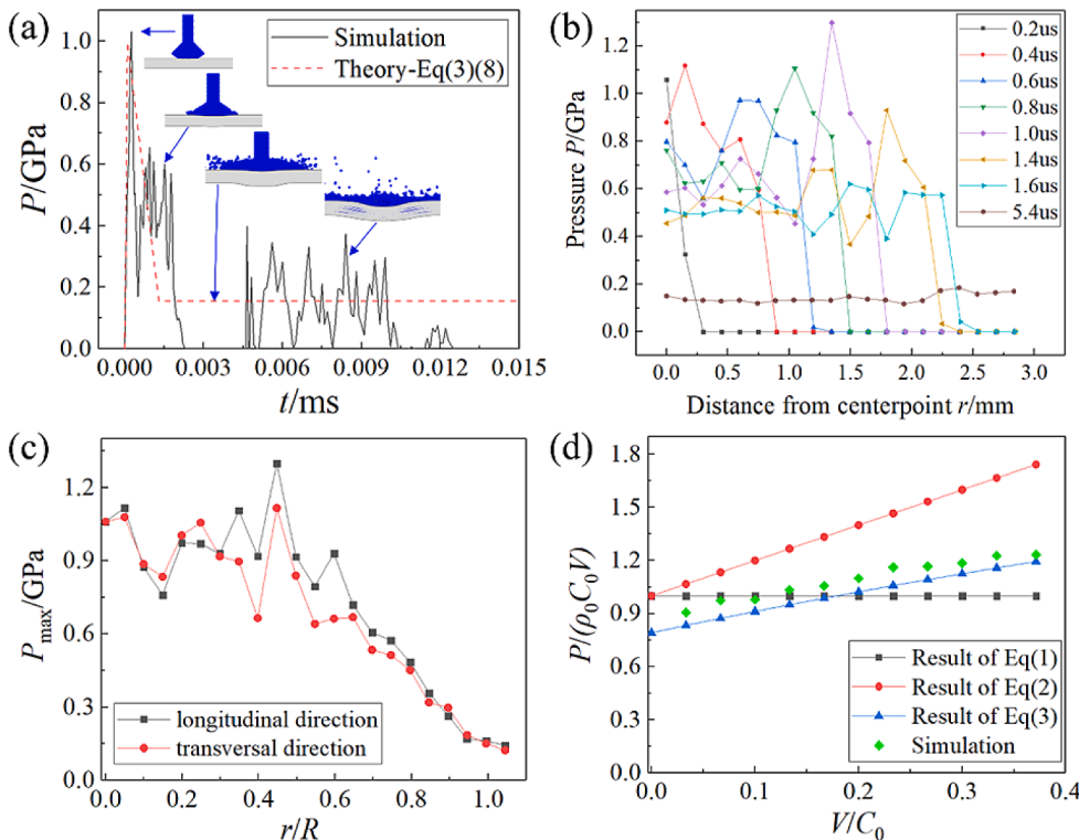
Fig 5. Simulation results of water-hammer pressure. (a) Time history of the water-hammer pressure of the center point on the CFRP surface impacted by a waterjet with the velocity of 557 m/s and the diameter of 6.2 mm. (b) Variation of the pressure distribution of the impacted surface as time progresses. (c) Maximum contact pressure distributed along both the longitudinal and transverse directions. (d) Normalized results of the peak impact pressure of the center point with respect to the impact velocity
