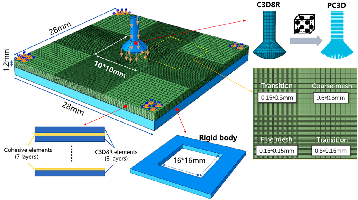
Fig 3. Finite element model of waterjet-CFRP laminate impact event
