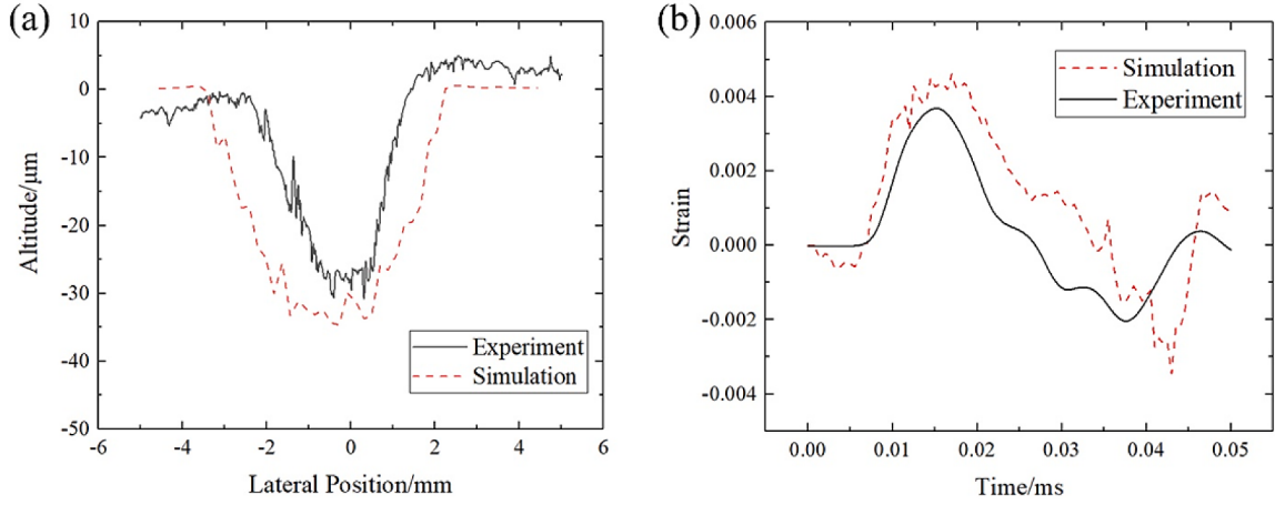
Fig 9. Simulation and experiment results of (a) profile of the impacted location and (b) time history of the strain at the back surface.
