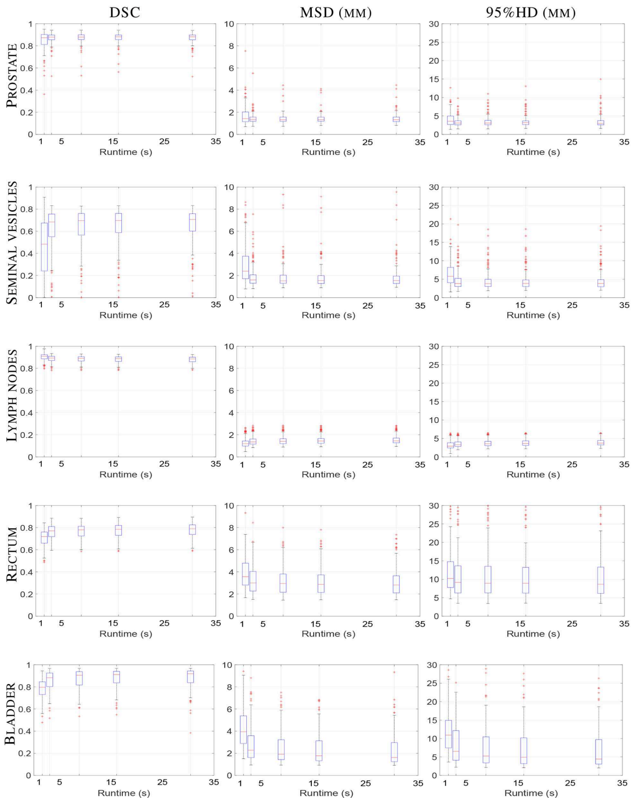
FIGURE 3 | Boxplot of elastix registration performance against runtime in seconds. From left column to right column the DSC (unit-less), MSD (mm) and 95%HD (mm) are shown, respectively. From top to bottom the prostate, seminal vesicles, lymph nodes, rectum and bladder are shown, respectively. Within one boxplot, from left to right the affine registration and B-spline registrations with 100, 500, 1,000, and 2,000 iterations are shown, respectively. Each boxplot contains results of 159 registrations.
