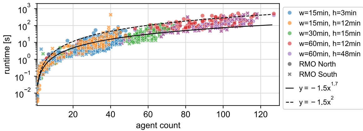
Figure 12. Runtimes of planning rounds over the number of agents
