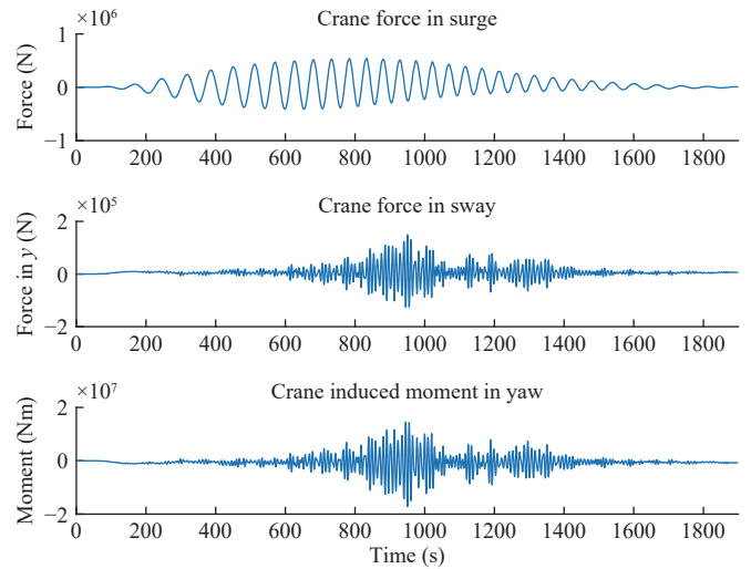
Fig. 11. Crane forces and moment in scenario S2 with PID controller, \vartheta = 3 .
