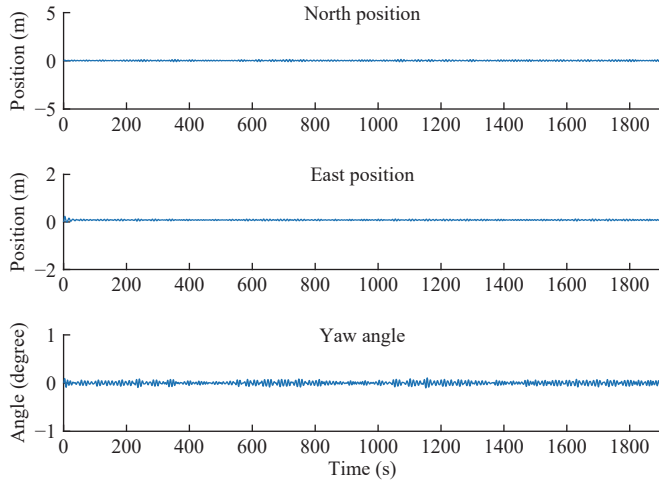
Fig. 4. Vessel position in scenario S1 employing the proposed controller.
