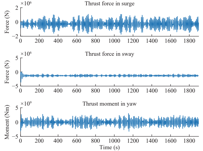
Fig. 6. Thrust forces and moment in S1 with the proposed controller.
