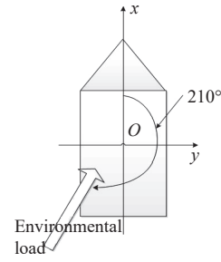
Fig. 2. Environmental load on the vessel.
