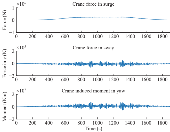
Fig. 8. Crane forces and moment in scenario S2 with the proposed controller, \vartheta = 3 .
