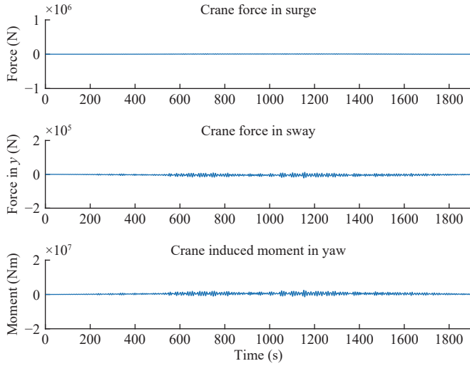
Fig. 5. Crane forces and moment in scenario S1 with the proposed controller.
