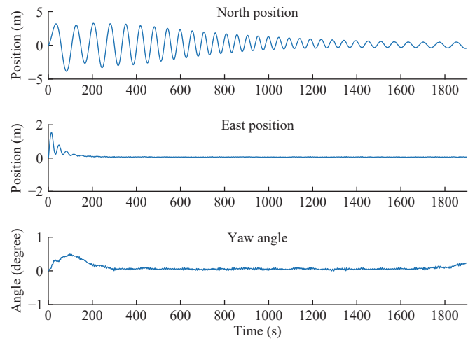
Fig. 10. Vessel position in scenario S2 with PID controller, \vartheta = 3 .
