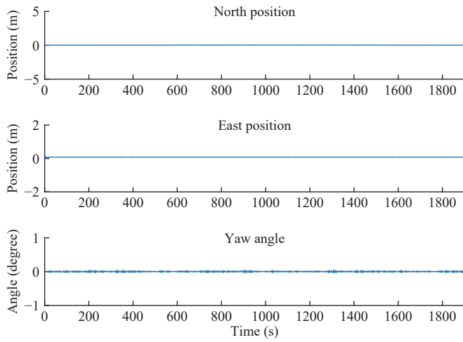
Fig. 7. Vessel position in scenario S2 with the proposed controller, \vartheta = 3 .
