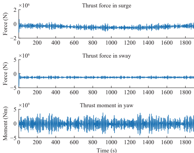
Fig. 9. Thrust forces and moment in S2 with the proposed controller, \vartheta = 3 .
