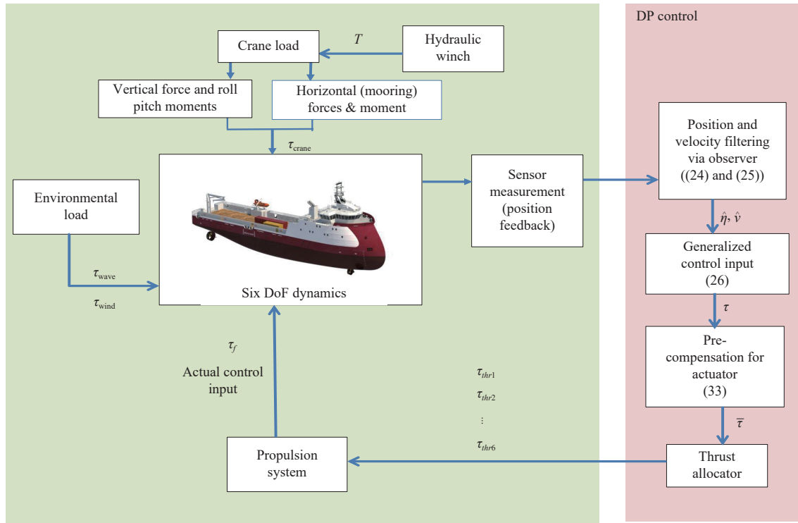
Fig. 1. Overall process plant model for the construction crane vessel. Unmodelled dynamics of the propulsion system affect the DP precision. Also, during offshore heavy lifting operation, instability of DP systems has been reported due to large mooring forces, which is the horizontal component of \tau_{\text{crane}} .
