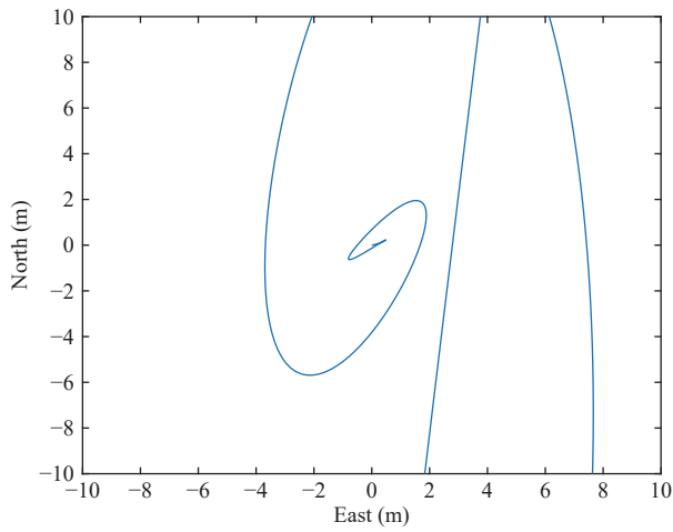
Fig. 12. Unstable behavior with controller from [26], \theta = 3 , due to neglecting propulsion dynamics.
