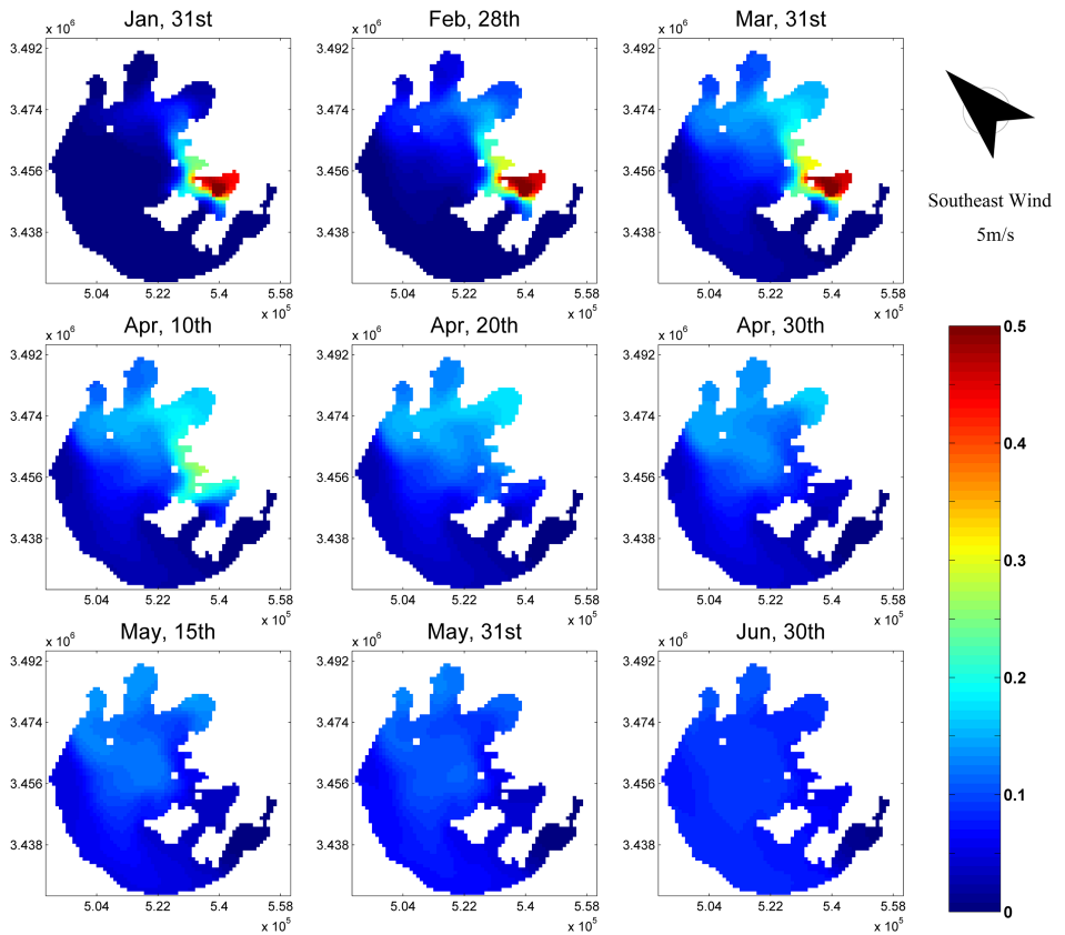
Figure 3.15: Time series of tracer concentration images, with the model driven by constant 5m/s south-east wind. Unit in the figure is kg/m^3 .
