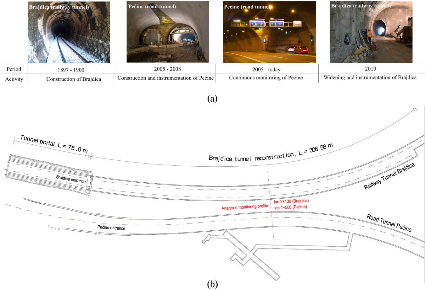
Fig. 6. Timeline of construction and monitoring (a) and layout (b) of two adjacent case study tunnels – railway tunnel Brajdica and road tunnel Pećine.
