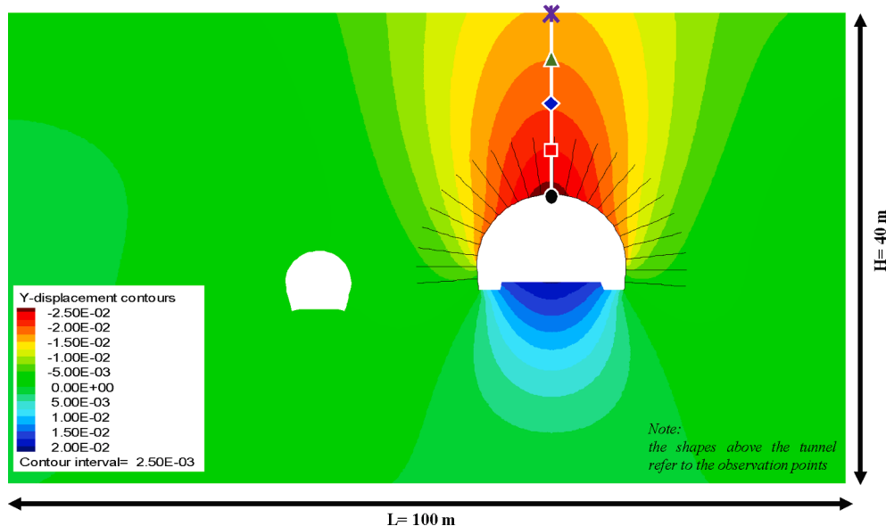
Fig. 9. Numerical model and contours of vertical displacements occurred shortly after the excavation of tunnel Pećine.
