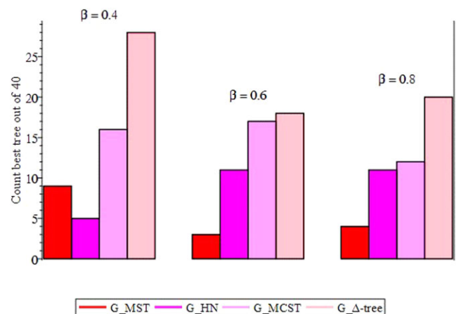
FIGURE 7 Bar chart of the number of times (out of 40) the best tree was found in sets 1-3, respectively
