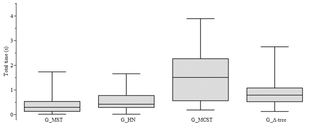
FIGURE C.3 Computational time needed to find Gilbert tree from four different spanning trees, including the time for generating the spanning tree
