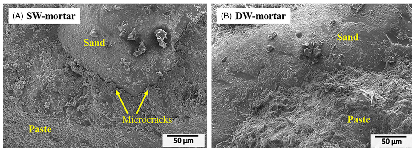
FIGURE 16 Morphologies of the seawater mixed AASF mortar (A) and distilled water mixed AASF mortar (B) after 56 days of curing based on SEM analysis. AASF, alkali-activated slag/fly ash. SEM, scanning electron microscopy
