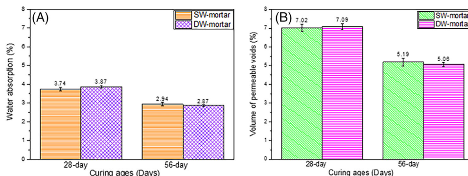
FIGURE 10 (A) Water absorption and (B) VPV of the seawater mixed mortar and deionized water mixed mortar after 28 and 56 days of curing. VPV, volume of permeable voids
