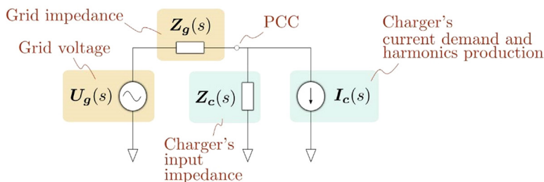
FIGURE 9.29 Impedance model of charger-grid system.
