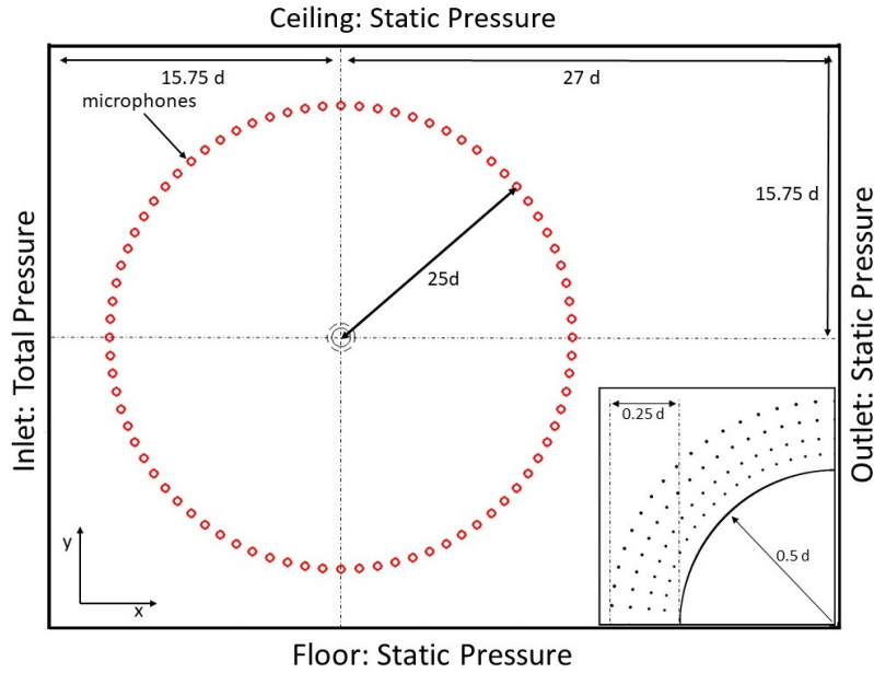
Fig. 3 Numerical setup designed to investigate the coated-cylinder flow-induced noise. An enlargement of the structured cover architecture is visible in the bottom-right corner. The microphone array used to compute the acoustic data is depicted in red.
