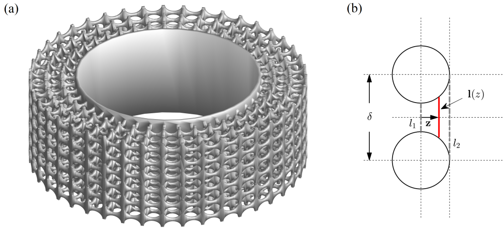
Fig. 14 (a) MATLAB .STL representation of a portion of an SPCC span and (b) schematic diagram of the vortex shedding element and the characteristic length term, l(z) .
