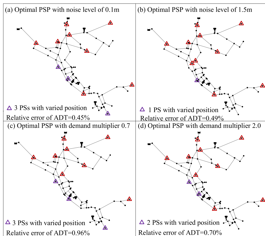
Figure 8. Optimal PSPs under varied noise levels and demand multipliers using the proposed method (reference PSP: Figure 5b).
