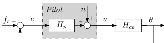
Fig. 1. Compensatory pitch tracking task.
