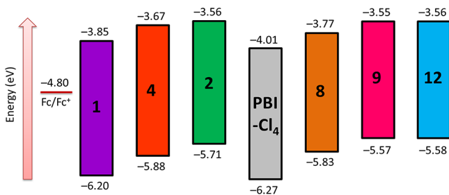
Figure 5. HOMO and LUMO levels of synthesized perylene derivatives against vacuum.
