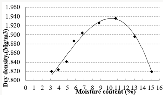
Figure 3: Modified proctor test result.
