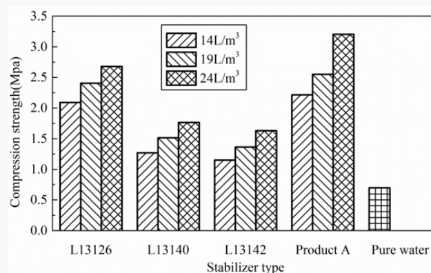
Figure 6: UCS values after 28 days curing.
