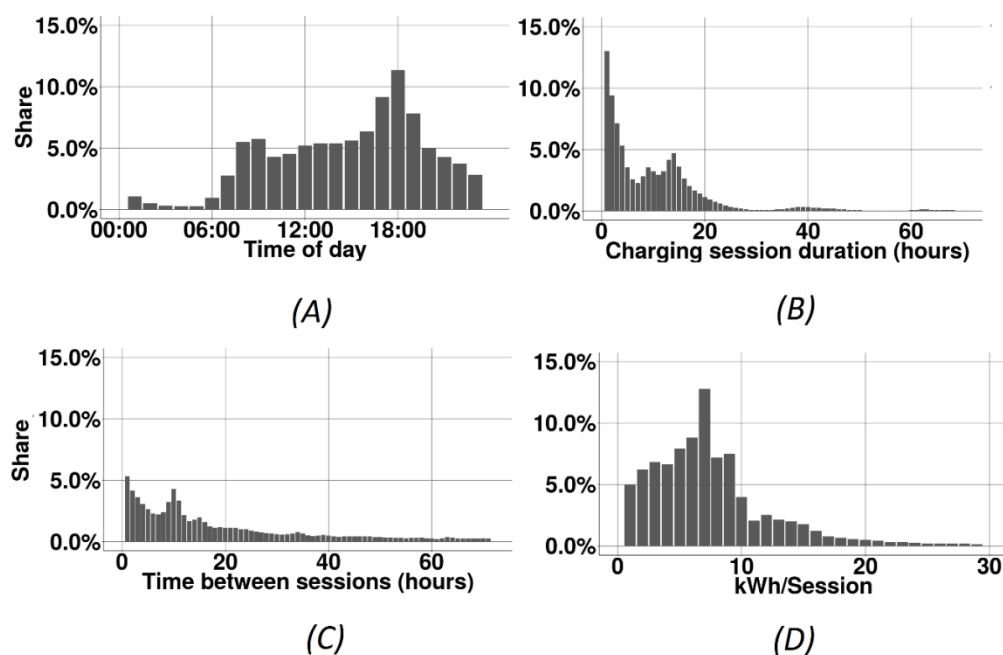
Figure 6.17 Charging patterns of agents, with (A) distribution of start times, (B) Connection duration and (C) Time between sessions and (D) kWh distribution
