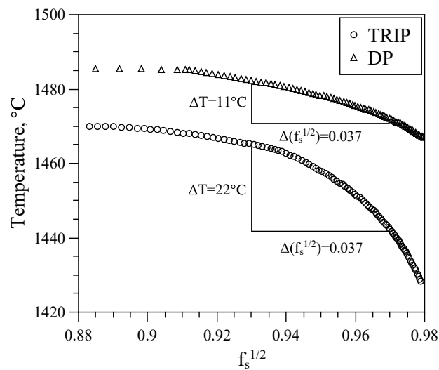
Fig. 12 Prediction of cracking susceptibility using the Kou criterion [9]. Slope of T - (f_s)^{1/2} curves with f_s varying from 0.87 to 0.94 indicates higher crack susceptibility of TRIP steel.
