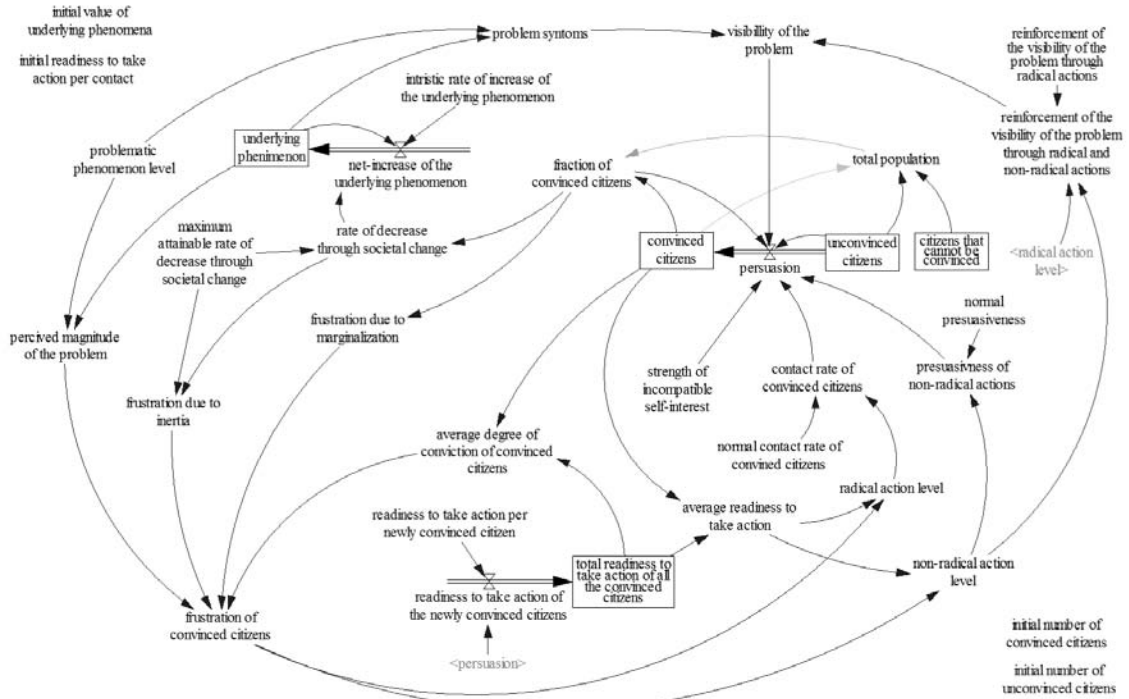
Figure 1: Stock-Flow Diagram of the generic de/radicalization model
