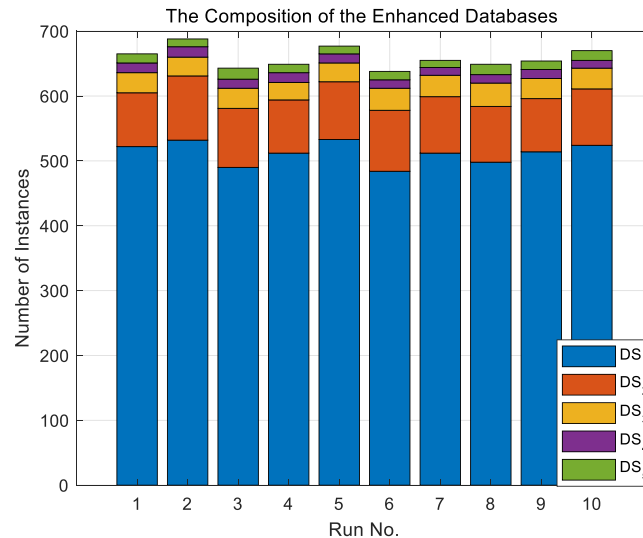
Fig. 6. The composition of the enhanced databases obtained from ten independent runs.
