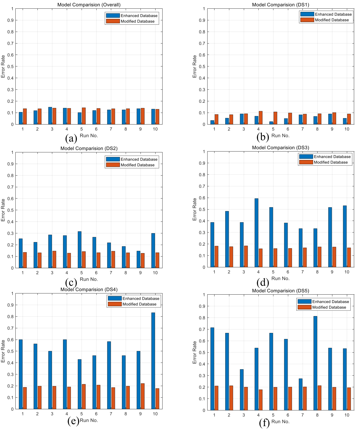
Fig. 10. Model Comparison ( \mathcal{C}_e vs \mathcal{C}_{em} ).
