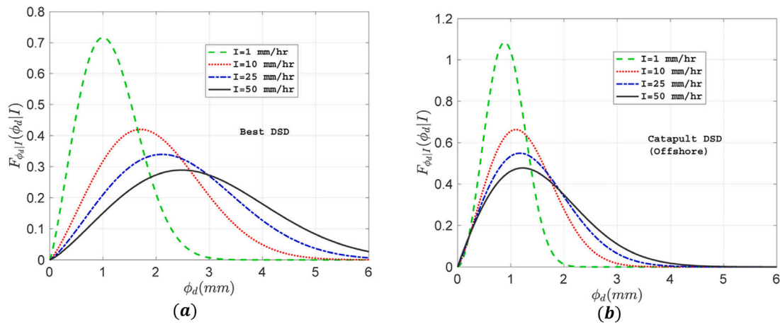
Fig. 11. (a) Onshore DSD (b) Offshore DSD. Source: Permission taken from [24].
