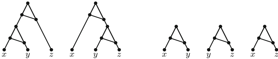
Fig. 1 An example of two level-1 trinetts (left) that display the same set of three binets (right). All arcs are directed downwards
