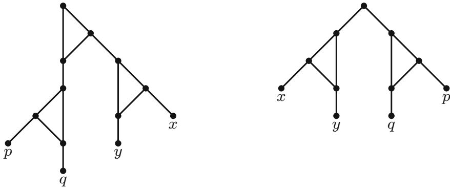
Fig. 5 Examples of two networks built recursively by using the operations introduced in the text
