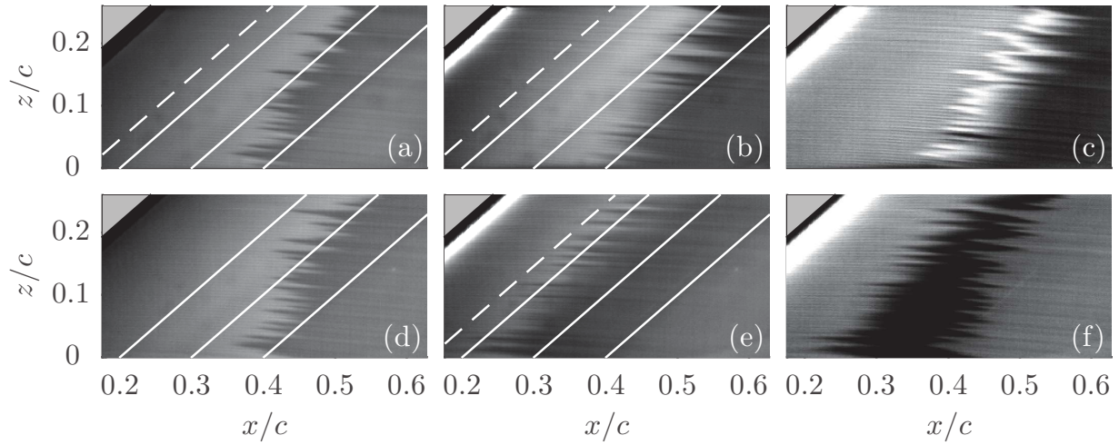
Figure 5: IR thermography mean fields ( Re_c = 2.1 \cdot 10^6 , U_\infty = 25\text{ms}^{-1} ). The flow comes from the left. The IR mean fields are dewarped and plotted in the xz plane. (a) Baseline (b) -F_x ( c_\mu = -0.71 ) (c) Subtraction of (a) from (b). (d) Baseline (e) F_x ( c_\mu = 0.71 ) (f) Subtraction of (d) from (e). The solid white lines represent constant chord positions. Dashed line at x/c = 0.15 refers to figure 6a.
