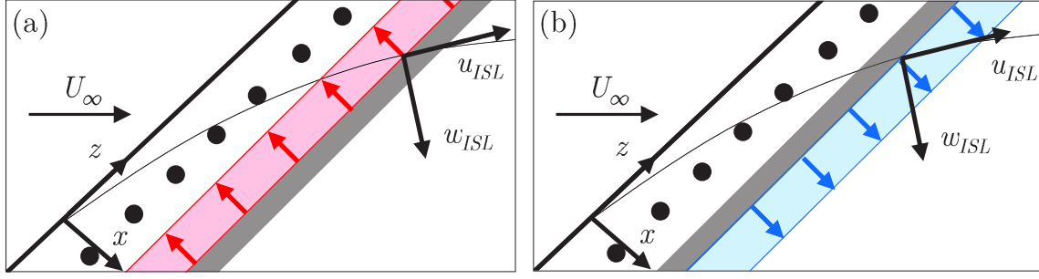
Figure 1: Schematic of the forcing mechanism (not to scale). Inviscid streamline (thin black line) and local velocity components ( u_{ISL} , w_{ISL} ). DRE arrangement (●) and plasma actuator exposed electrode (grey bar). (a) -F_x plasma forcing (red arrows) (b) F_x plasma forcing (blue arrows).
